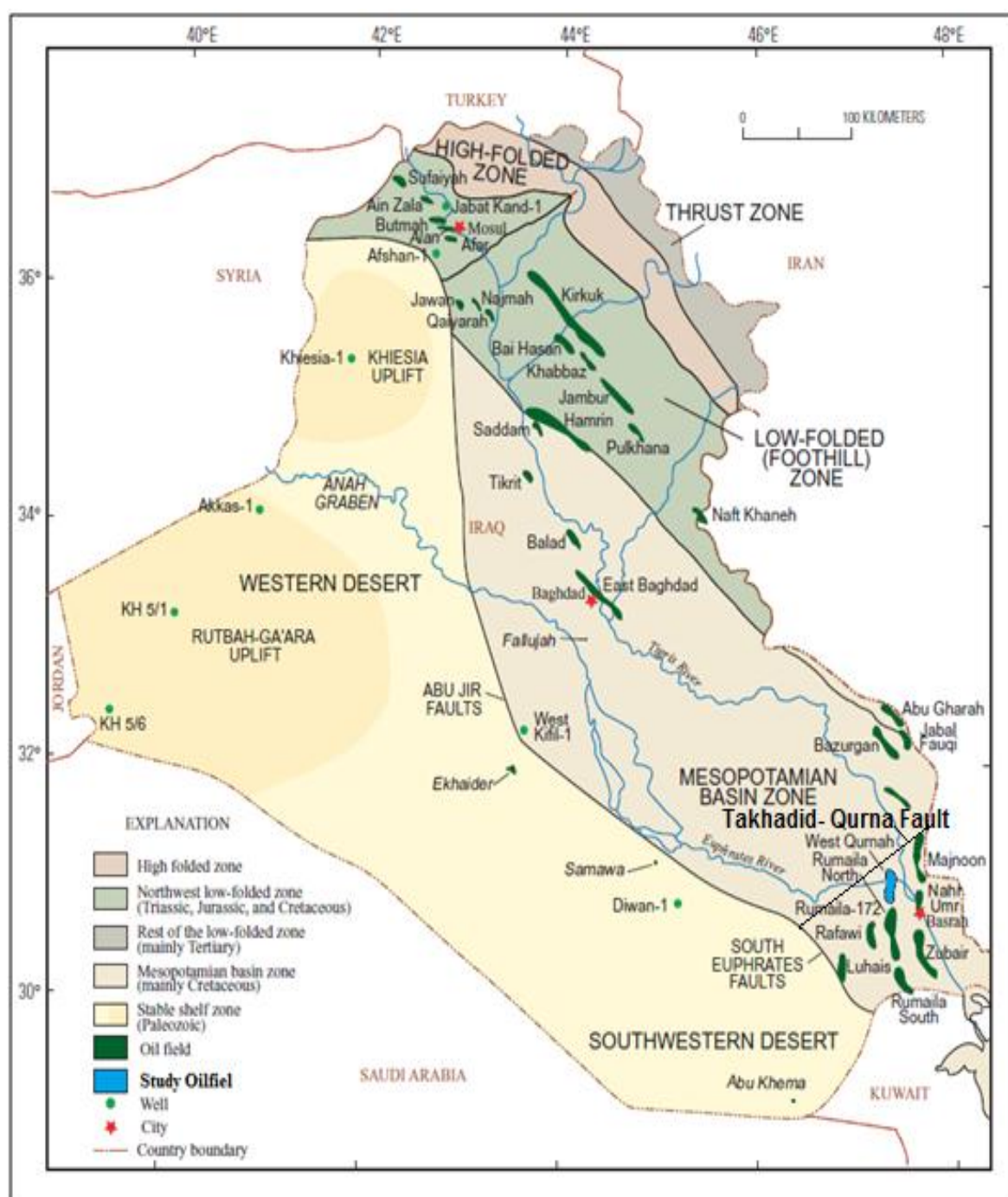
Figure 1- Map showing location of Mesopotamian Basin and Zagros fold belt. The Zubair subzone bounded in Iraq with Takhadid-Qurna and South Euphrates faults [5]
