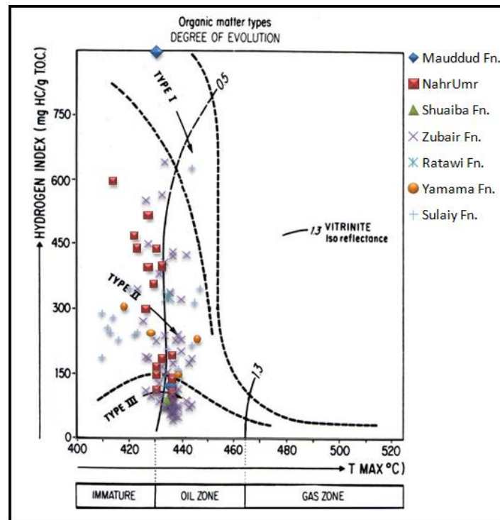
Figure 3- The kerogen types, product zone and maturity in terms of HI, Tmax, and Ro in Lower Cretaceous formations [10].
