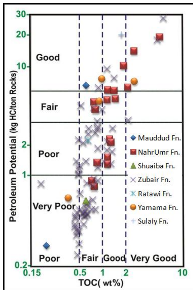
Figure 5- Source rock potential interpretation by plotting PP vs. TOC modified from [11] in Lower Cretaceous formations, the cross plot assigned to the prospectivity of the formations.
