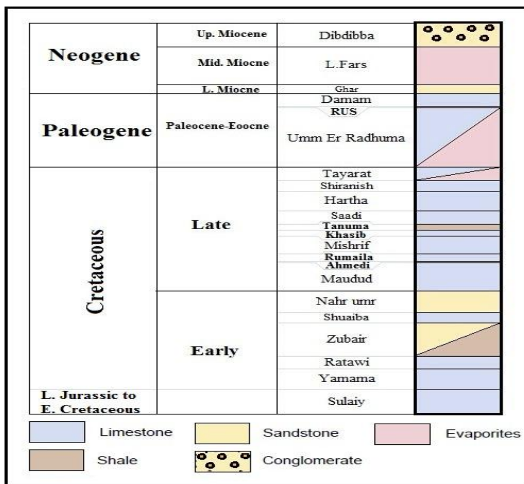
Figure 2- A stratigraphic section to the succession of the Cretaceous and Cenozoic in West Qurna Oilfield.
