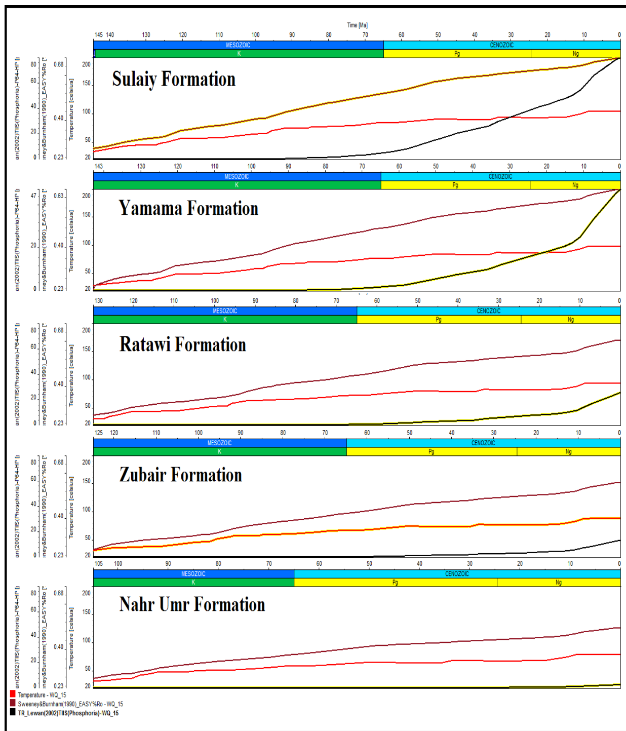
Figure 9- Temperature (the red curves), vitrinite reflectance (the dark red curves), and transformation ratio (the black curves) in well WQ_15.
