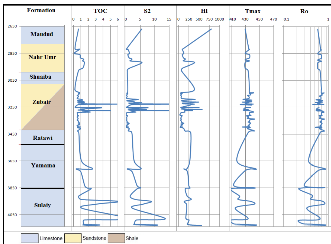
Figure 7- a geochemical log shows the studied intervals in terms of TOC, S2, HI, Tmax, and Ro.
