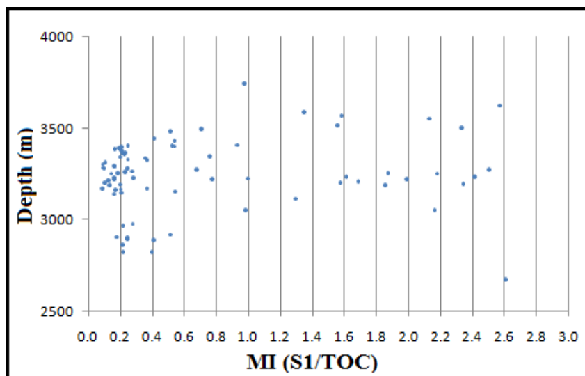
Figure 6- Cross plot of depth versus migration index (S1/TOC or Expulsion efficiency diagram), show the good efficiency of the studied formations.
