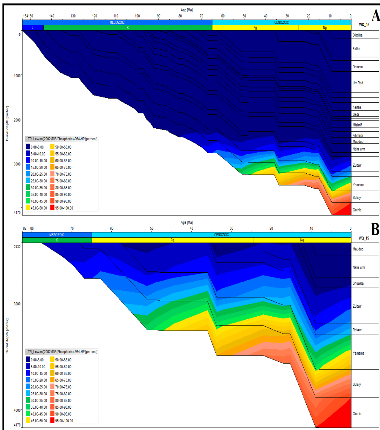
Figure 8- A- Represents the burial history curves, superimposed by the transformation ratio (TR) representing TR of the organic matters into HC. B- Close section to the L. Cretaceous succession in WQ_15 well.
